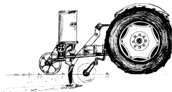
Figure 11. A pocket gopher burrow builder. The burrow builder meters out grain bait into an artificial burrow. Pocket gophers enter the artificial burrow where it intersects the natural burrow and find the bait.
